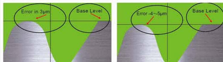
Linear Motor (Radius Error: 3µm) by optical projection 120X Ball Screw (Radius Error: 4-5µm) by optical projection 120X
